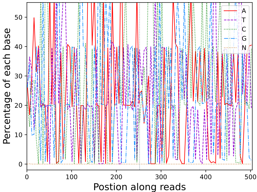
Base percentage along reads (R20101)
